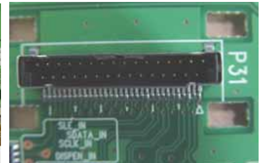
Signal input(LVDS)
